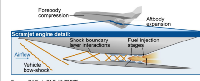
Figure 2. Scramjet Engine. The air enters the inlet at a speed greater than Mach 1. It is then compressed by the engine geometry, and combustion occurs at supersonic speeds.
