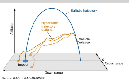
Figure 1. Ballistic Reentry Vehicle (RV) Versus HGV Trajectories. An RV follows a parabolic trajectory determined mainly by its launch characteristics, its target, and gravity. An HGV can take a variety of trajectories and leave its final destination ambiguous.
