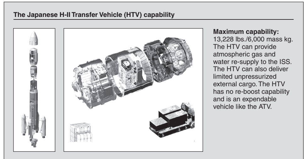
Figure 6: The Japanese H-II Transfer Vehicle (HTV)
