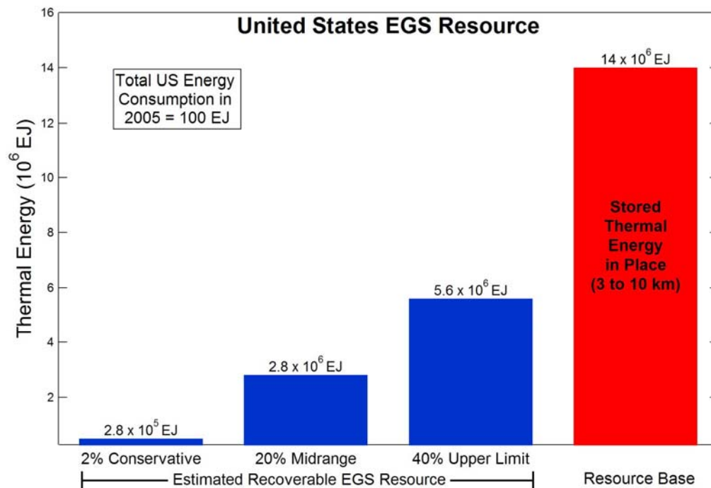
Figure 2. Estimated total U.S. geothermal resource base and recoverable resource the 40% upper limit is based on the analysis of Sanyal and Butler (2005) while lower recoverable amounts are estimates from The Future of Geothermal Energy , MIT report, 2006.
